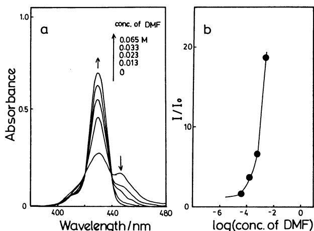
Fig. 5. The dependence of Soret absorption spectra (a) and I/I_0 (b) for 1.7 \times 10^{-6} M \text{ZnPC}_2\text{bpy}^+(3) in o -DCB on the concentration of DMF at room temperature, where I and I_0 denote the fluorescence quantum yields in the presence and the absence of DMF at the excitation wavelength of 420 nm (isosbestic point).
