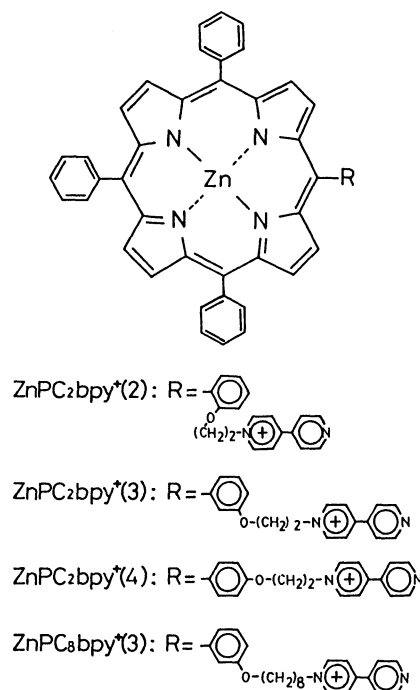
Fig. 1. Structures and abbreviations of zinc porphyrins.
