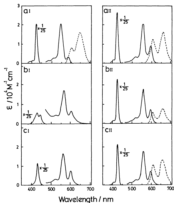
Fig. 2. Absorption (—) and fluorescence (----) spectra of ZnTPP (a), \text{ZnPC}_2\text{bpy}^+(3) (b) and \text{ZnPC}_8\text{bpy}^+(3) (c) in o -DCB(I) and DMF(II) at room temperature.
