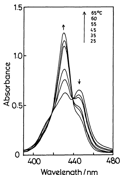
Fig. 4. Temperature-dependence of Soret absorption spectra of 4.1 \times 10^{-6} M ZnPC 2 bpy + (3) in o -DCB.
