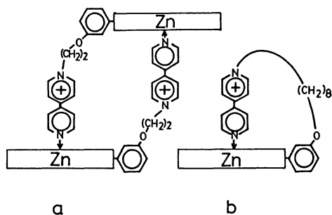
Fig. 3. Typical schematic axial coordination models of ZnPC 2 bpy + (3) (a) and ZnPC 8 bpy + (3) (b). □ Denotes porphyrin ring, and N→Zn coordination between Zn and N(pyridyl group).
